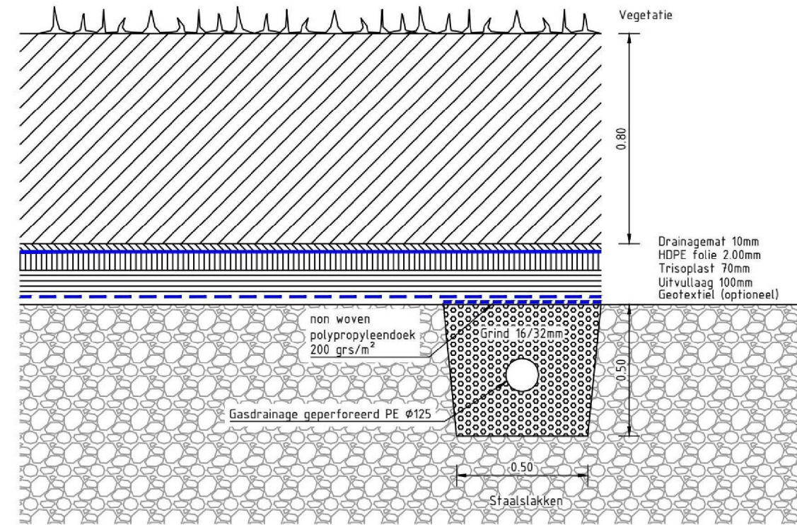
Detail horizontale gasdrainage Schaal 1:20
