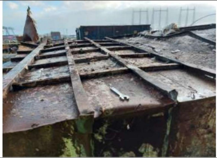
Description photo: 15-3-2021 parts off separation between FGD and Precips
