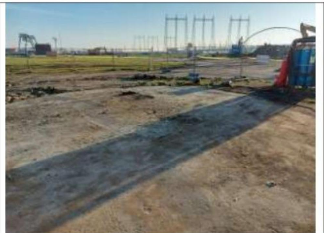
Description photo: clean concrete floor after removed the asbestos stamps and textile bandage
