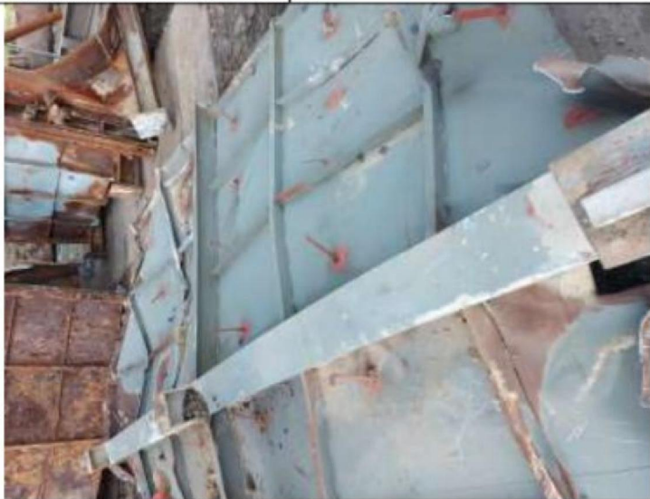
Description photo: 25-3-2021 parts off separation between FGD and Precips
